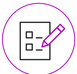
Supplier Onboarding
