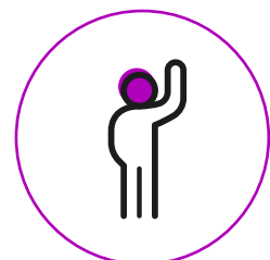
Leavers Processes
